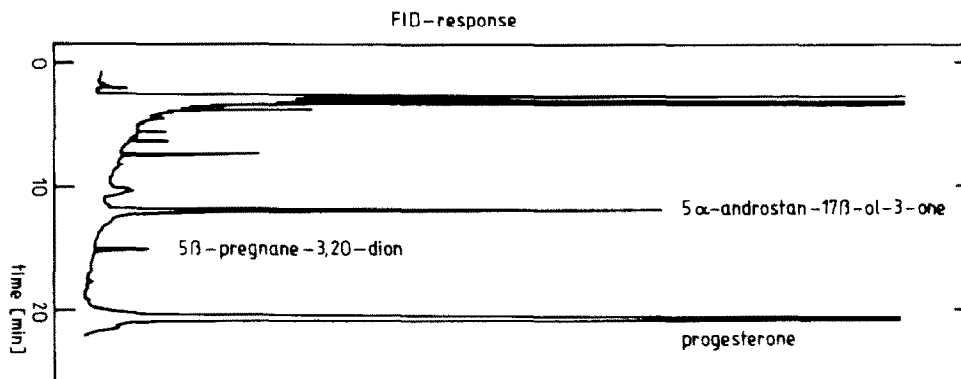
Fig. 2. Gas chromatogram of a standard enzyme assay. The enzymic product 5β-pregnane-3,20-dione (RRT: 1,281), was formed in vitro. Progesterone was used as substrate of the enzymic reaction and 5α-androstan-17β-ol-3-one (100 mM) as internal standard. Further confirmation of product identity came from g.c./m.s. data.
